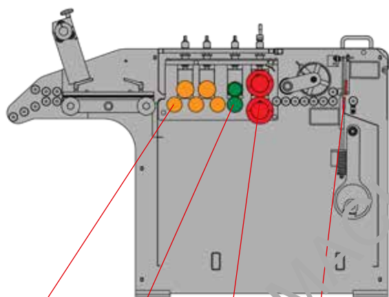
Straightening rolls Feeding rolls Slitting unit Mechanical shear
