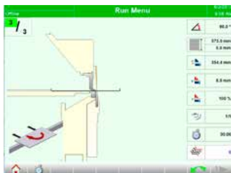
Shows the folding sequence and how to handle the material.
